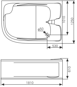
G9027(Right) Right Skirt Panel: you will see the bathtub installed against a RIGHT corner of the wall when you face to it.
